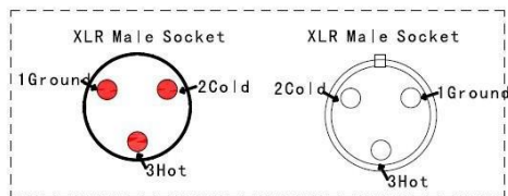
XLR Pin Configuration
